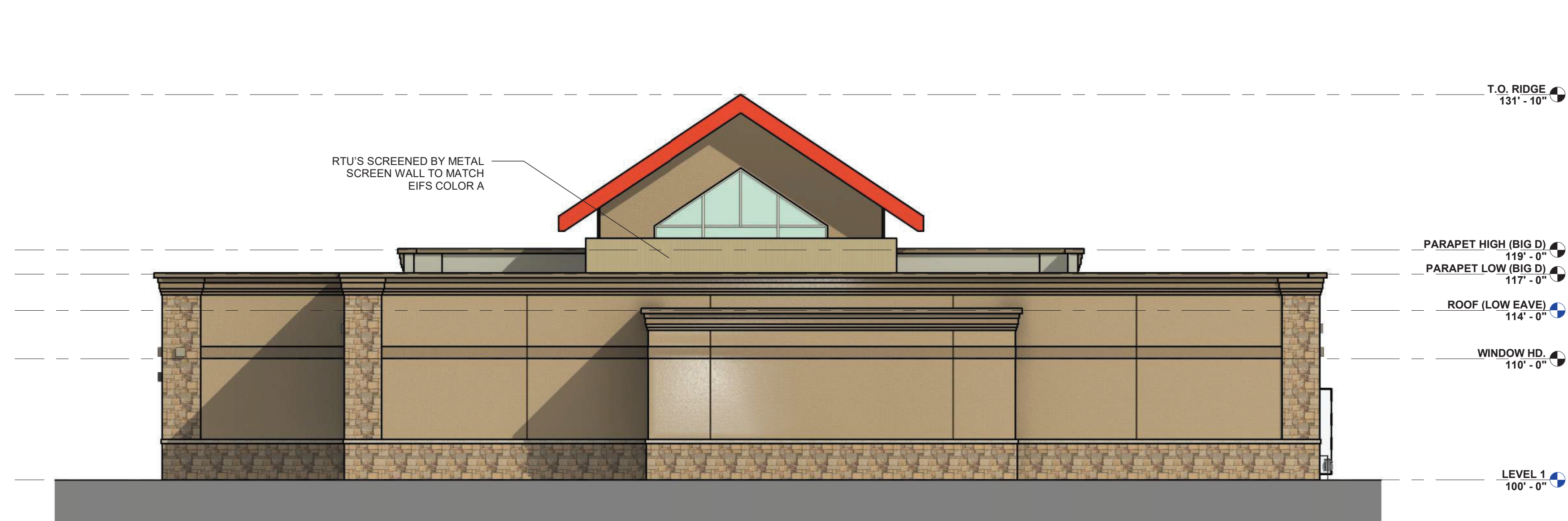
2 SOUTH ELEVATION - BIG D OIL - COLOR 1/8" = 1'-0"
